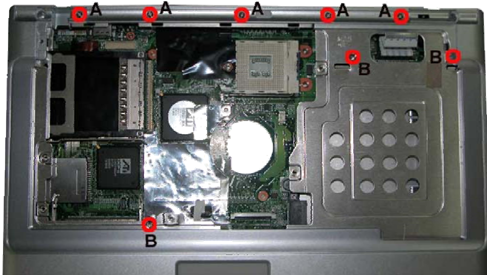
Fig. 25 Top Cover screws
